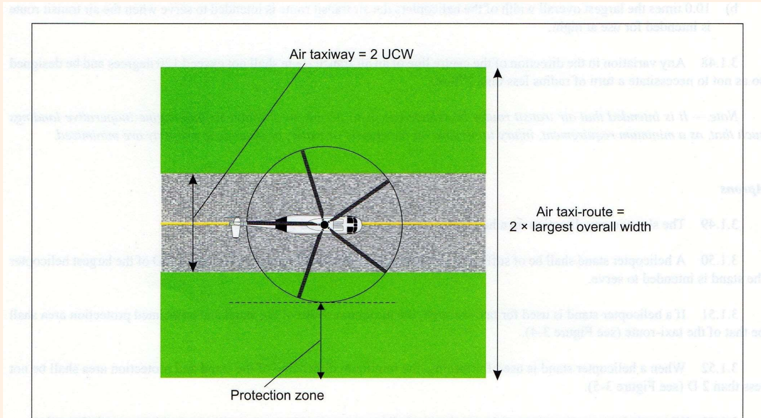
Figure 3-3. Air taxi-route
