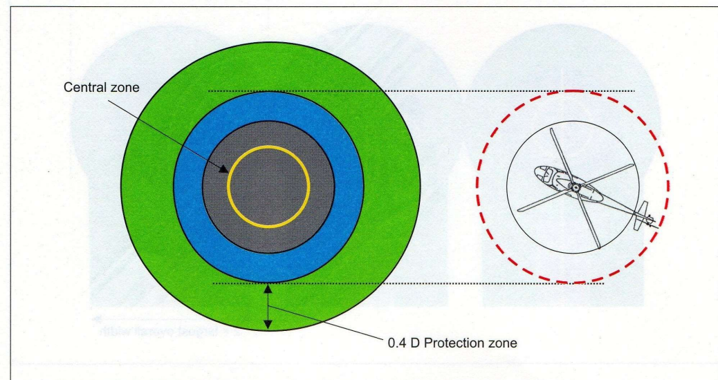
Figure 3-5. Helicopter stand protection area
