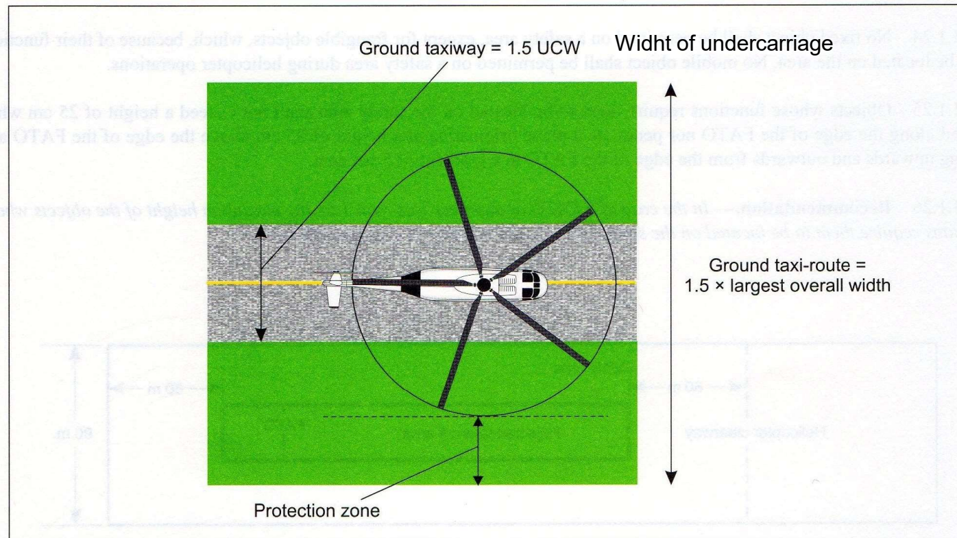
Figure 3-2. Ground taxi-route
