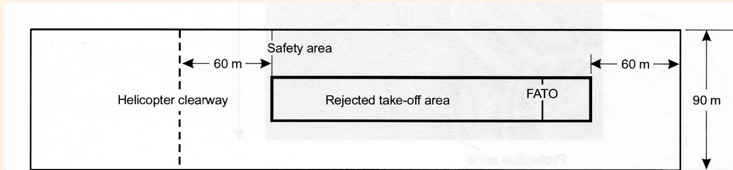
Figure 3-1. Safety area for instrument FATO
