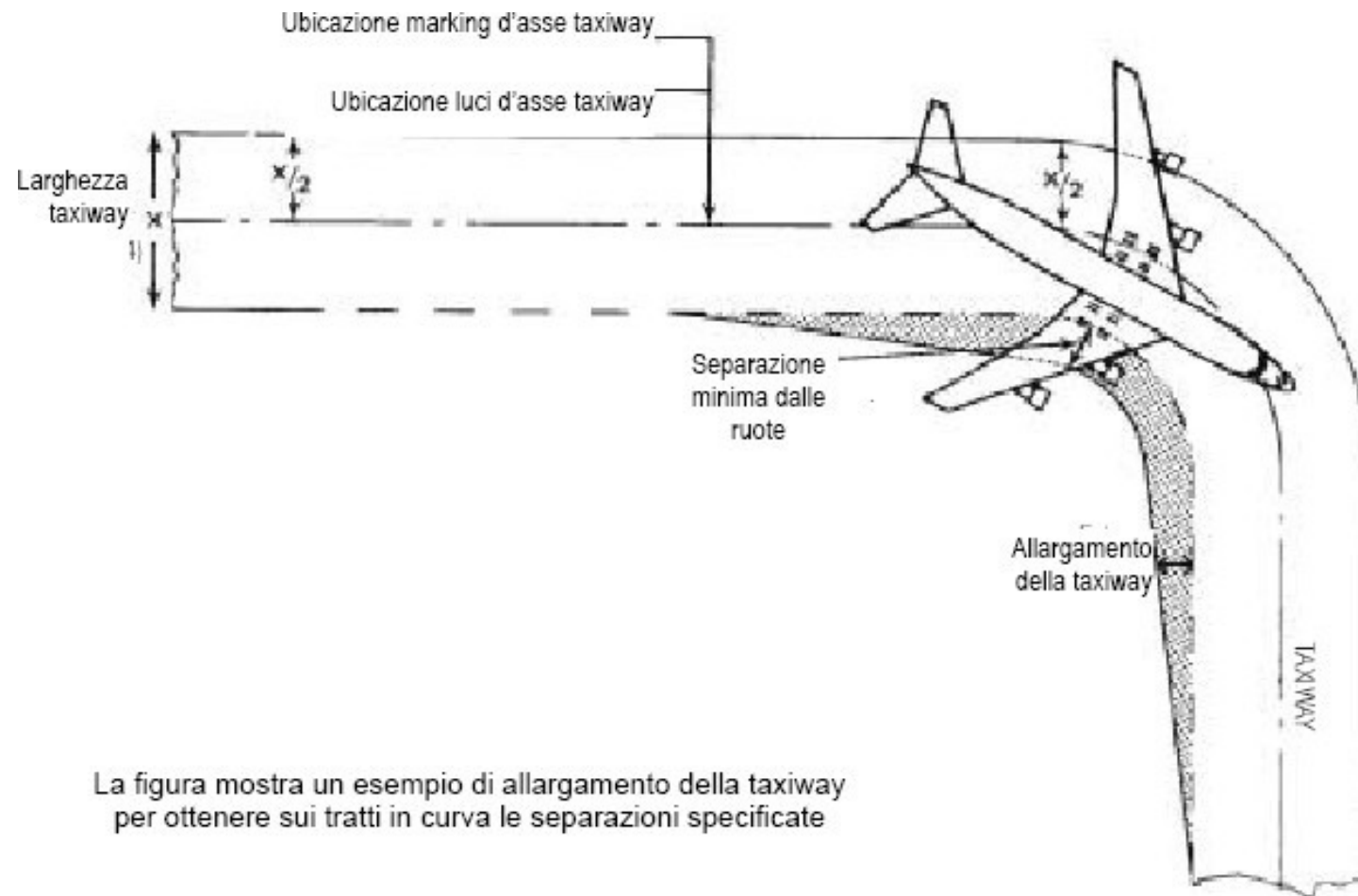
Allargamento taxiway in curva
